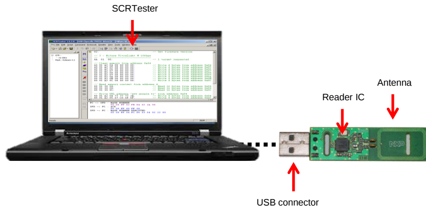
Example: PNEV553D demoboard
