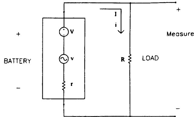
Figure 4: Low Frequency Chemical Battery Circuit Model
