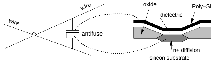
Figure 6 - Actel Antifuse Structure.
