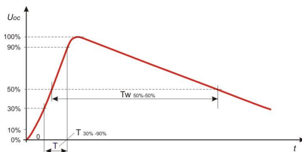
Voltage impulse TSurge
