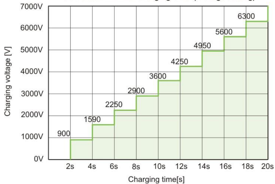
UCS 500N7 minimal charging time f( voltage setting)
