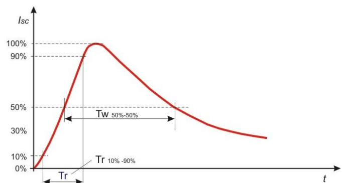
Current impulse TSurge
