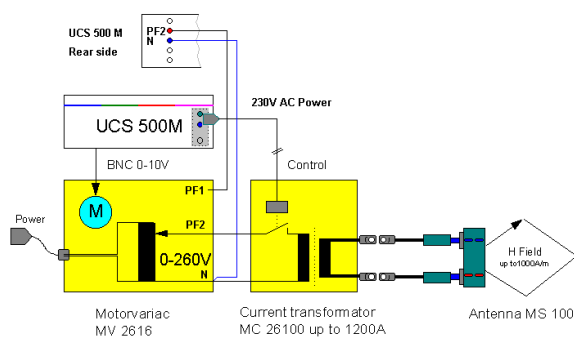
Schematics
