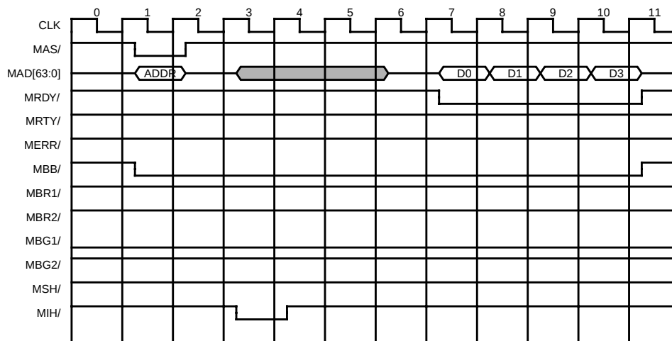
Waveform 22 Coherent Read and Invalidate (of Owned Data)
