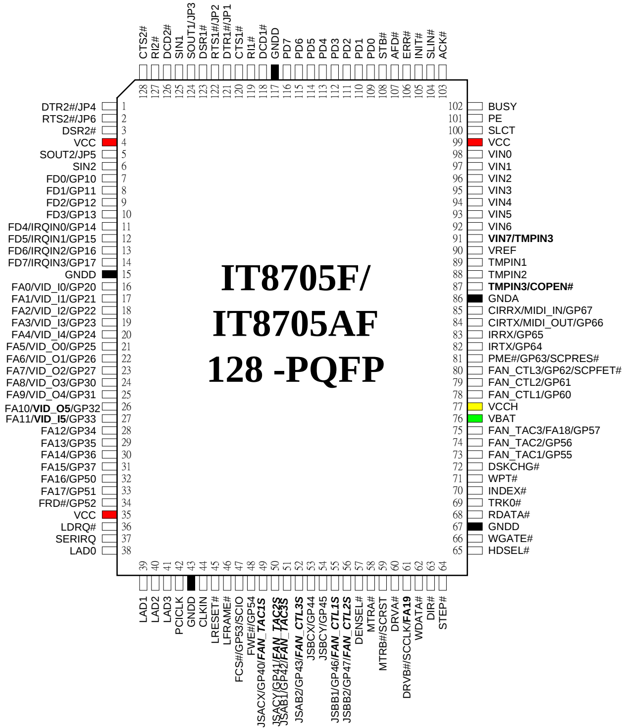
Top View
