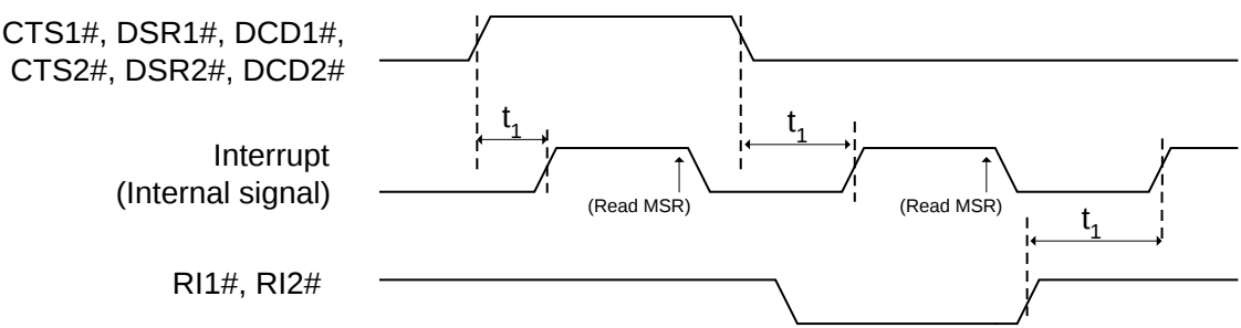
Figure 11-5. Modem Control Timings
