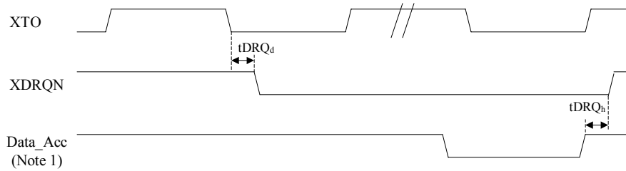
Fig. 8-3 Data Access Request Timing Characteristic.
