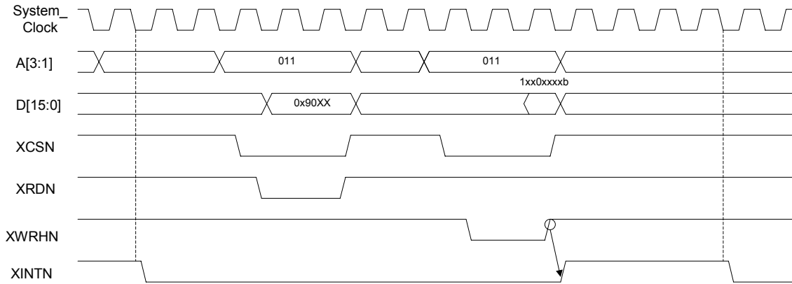
Fig. 7-10 Timing of Interrupt in (XINTN pin goes to low again).
