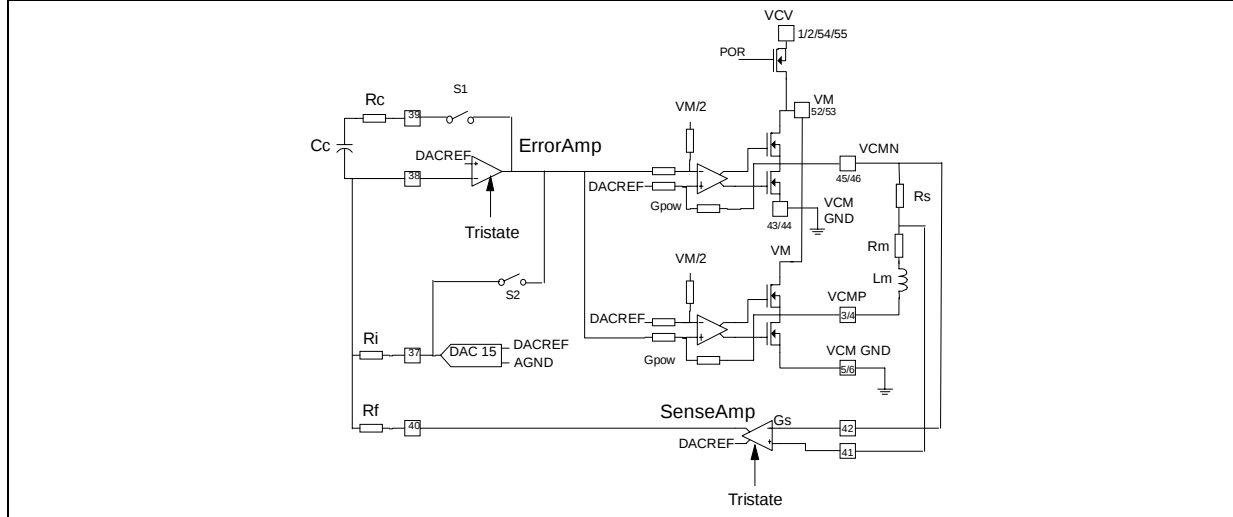
Figure 7. VCM Driver Block Diagram
