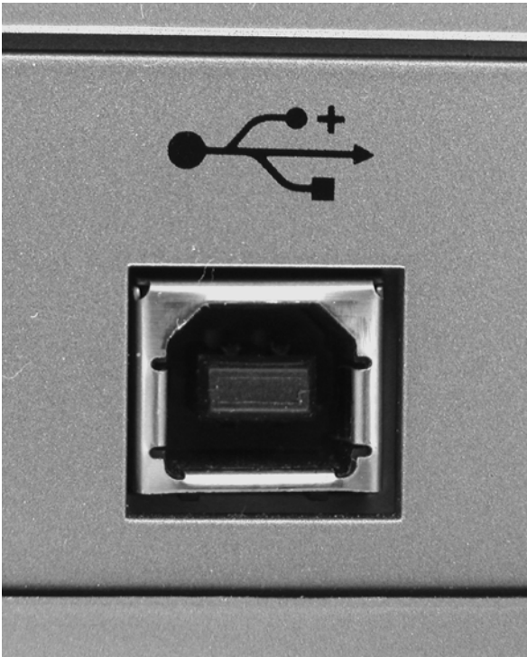
Figure 19-8: The USB icon identifies a USB plug or receptacle. A “+” indicates support for high speed.
