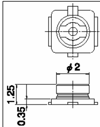
Figure 32: Mechanical dimensions of MC55i-W antenna connectors
