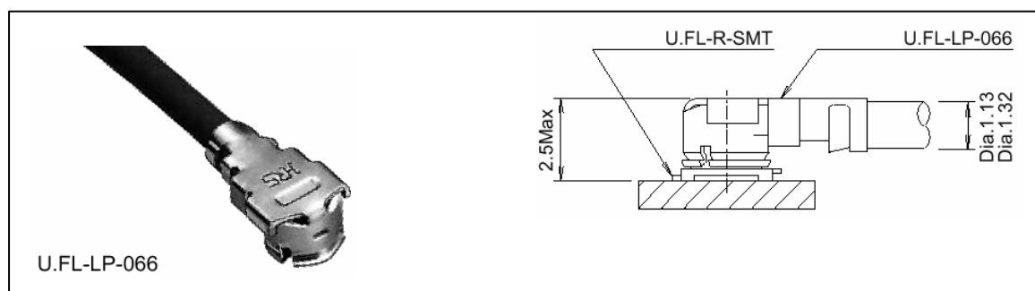
Figure 34: U.FL-R-SMT connector with U.FL-LP-066 plug
