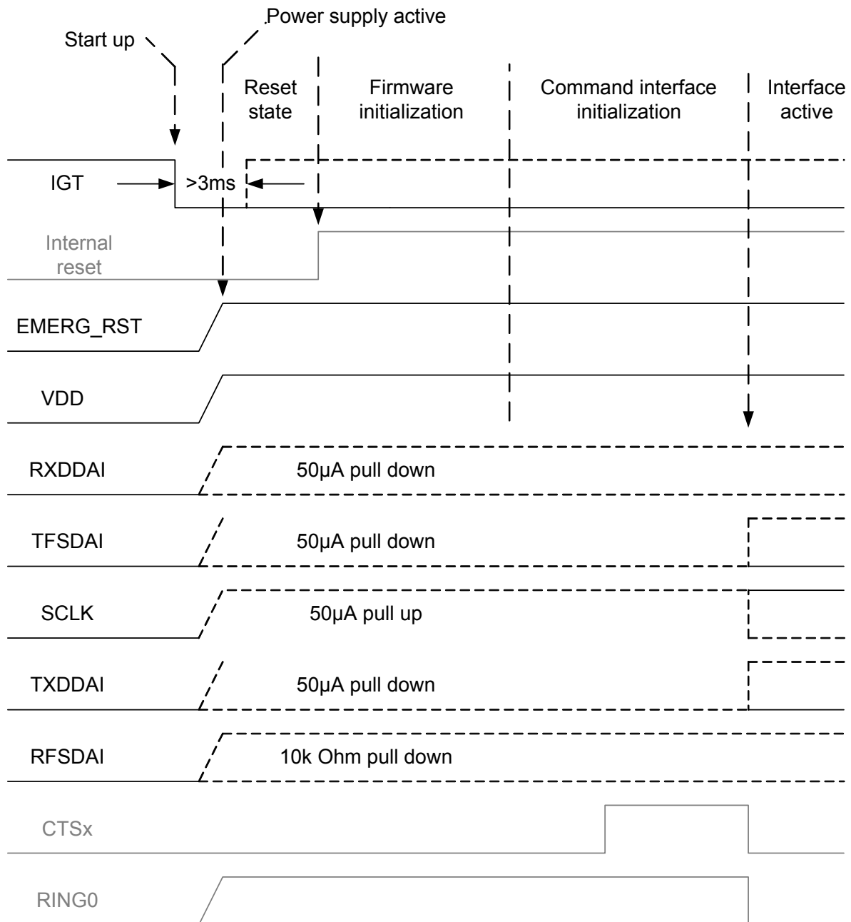
Figure 25: DAI startup timing
