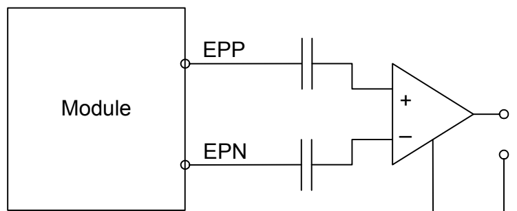
Figure 23: Line output connection
