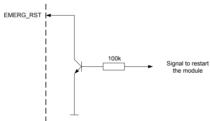
Figure 8: EMERG_RST circuit
