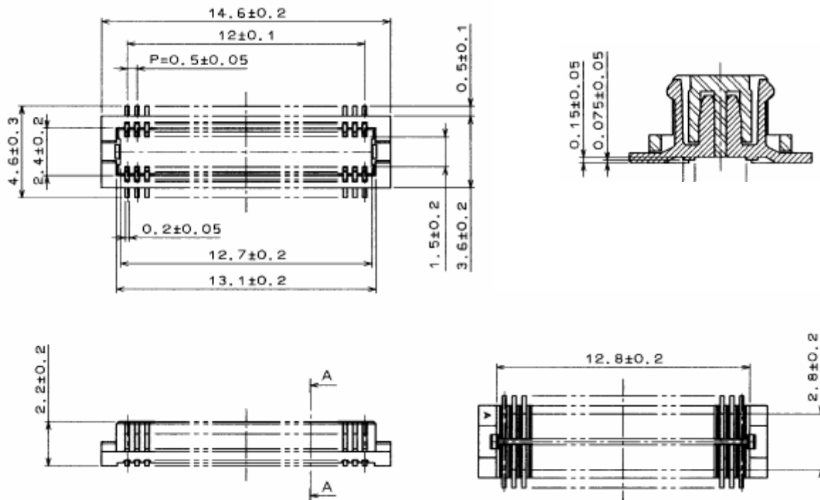
Figure 41: Mechanical dimensions of Hirose board-to-board connector
