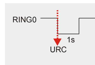
Figure 29: URC transmission
