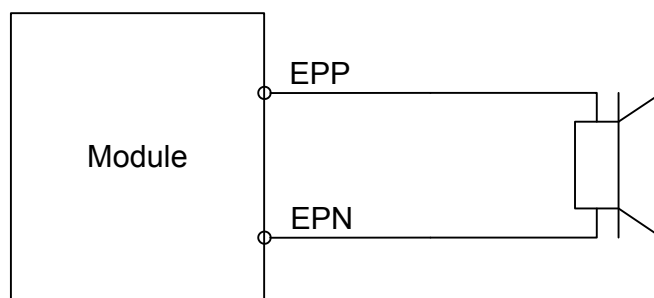
Figure 22: Differential loudspeaker connection
