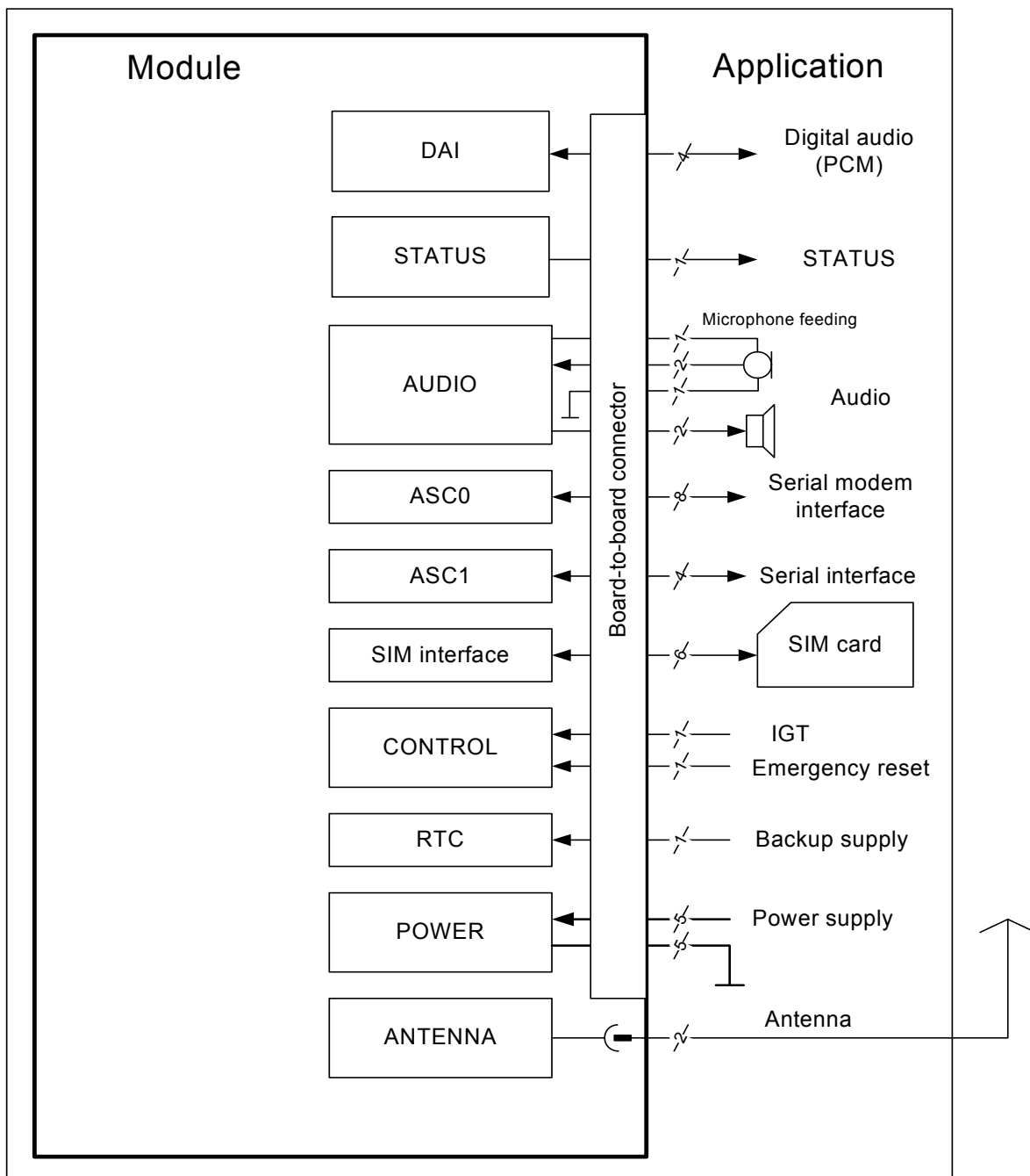
Figure 1: MC55i-W system overview
