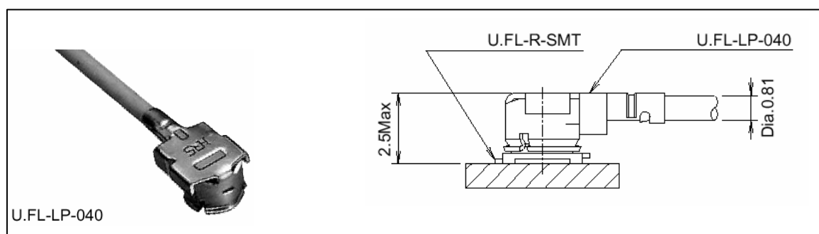
Figure 33: U.FL-R-SMT connector with U.FL-LP-040 plug
