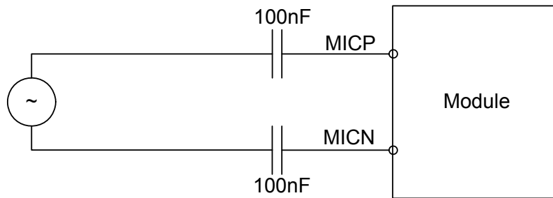
Figure 21: Line input
