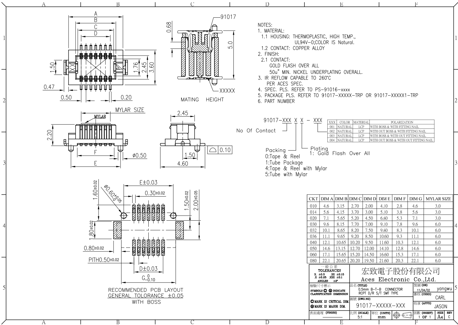
Figure 42: Mechanical dimensions of ACES board-to-board connector
