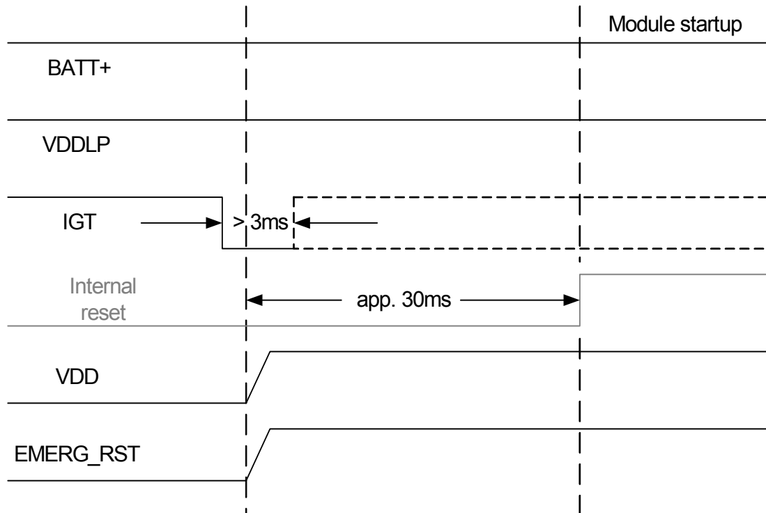
Figure 6: Power-on by ignition signal
