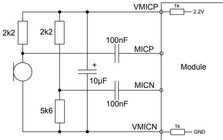
Figure 19: Single ended microphone connection
