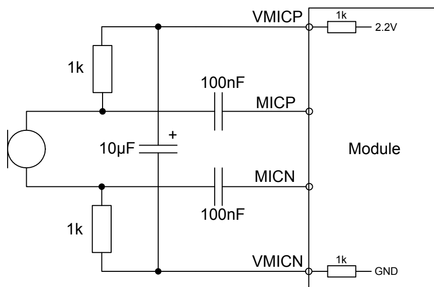
Figure 20: Differential microphone connection
