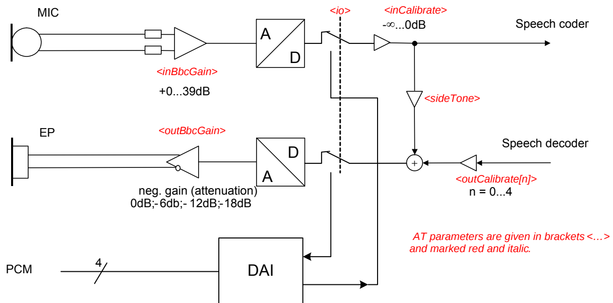
Figure 37: Audio programming model
