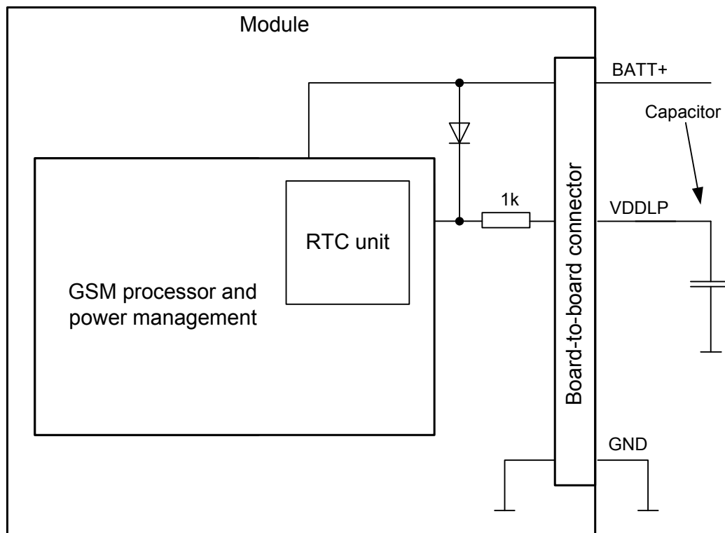
Figure 13: RTC supply variant
