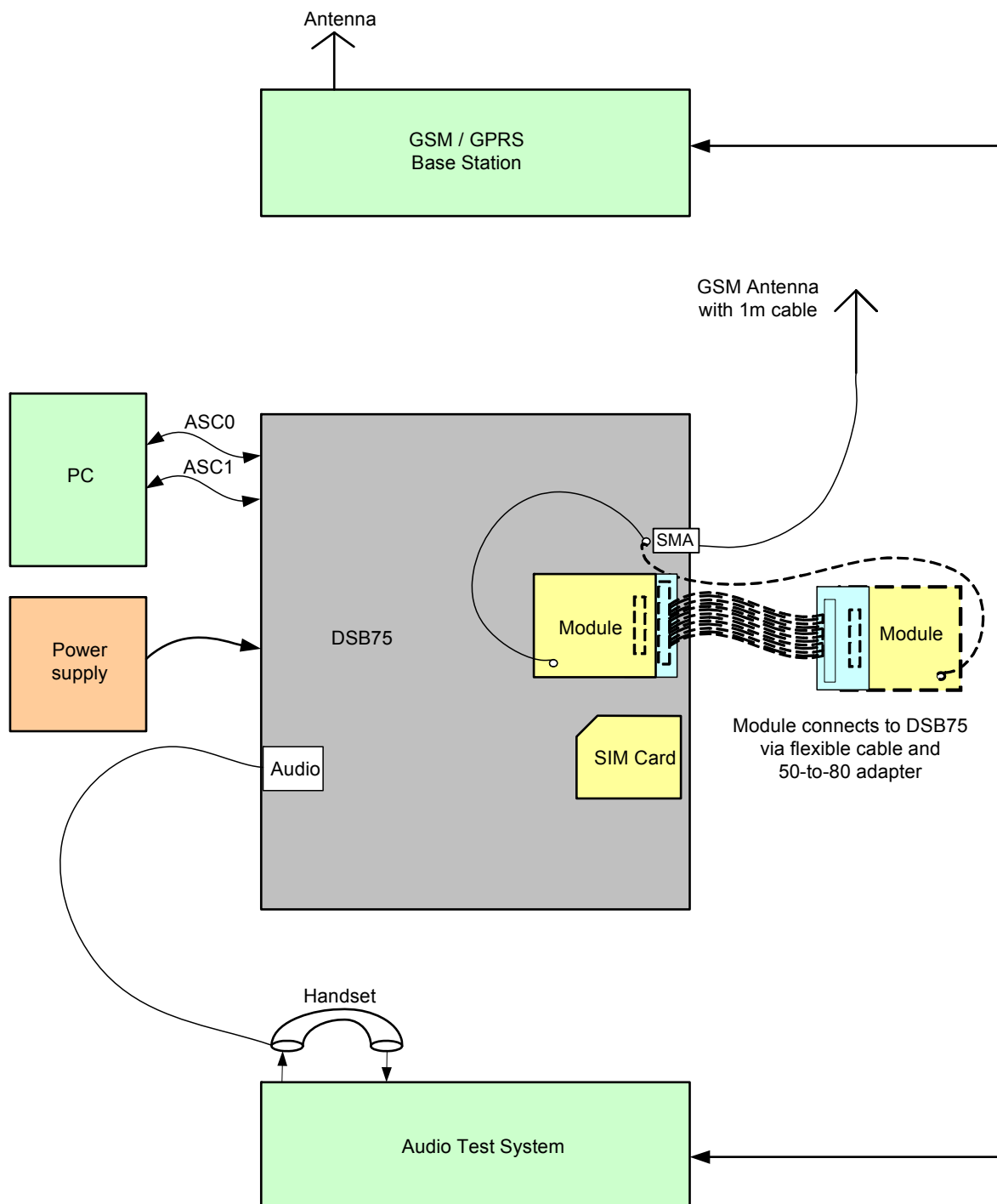
Figure 43: Reference equipment for approval
