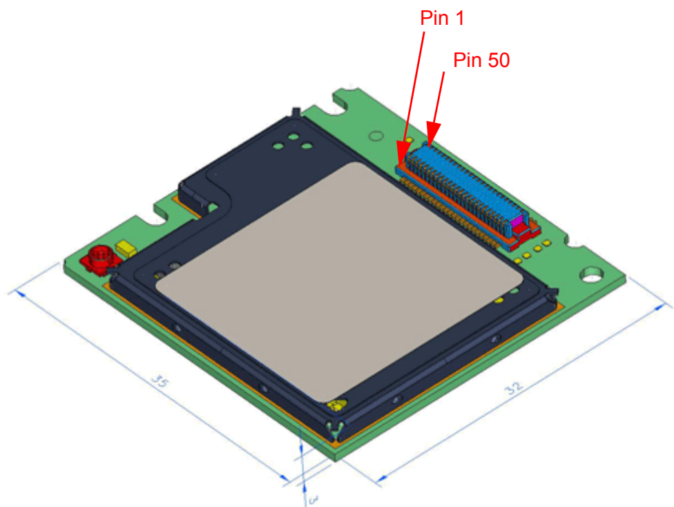
Figure 38: MC55i-W – top view
