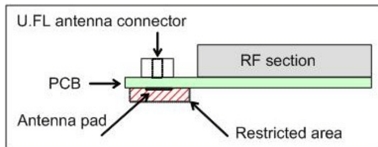
Figure 31: Restricted area around antenna pad
