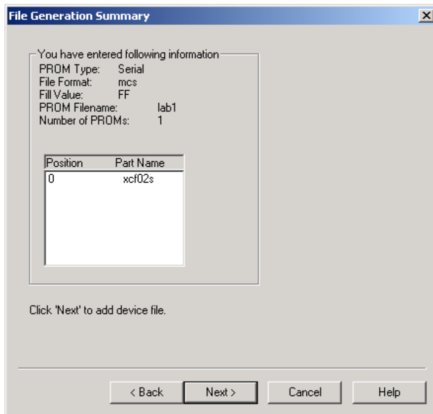
Figure 41: Summary Window
