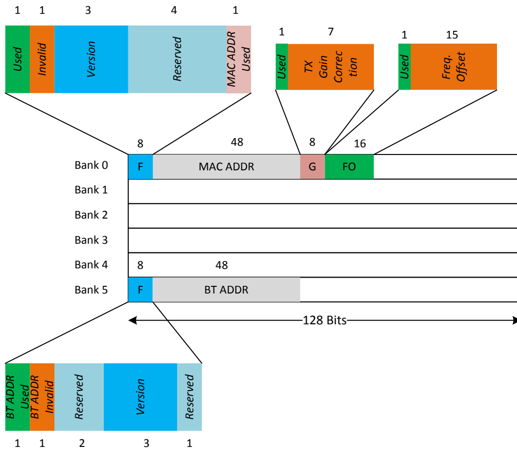
Figure 7-1. ATWILC3000 eFuse Bit Map
