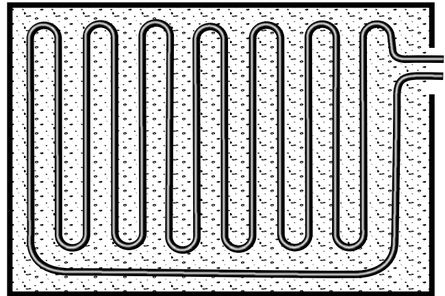
Fig. 6.7: Serpentine pipe layout
