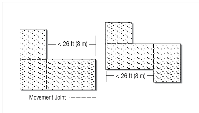
Fig. 5.4: Location of thermal mass joints
