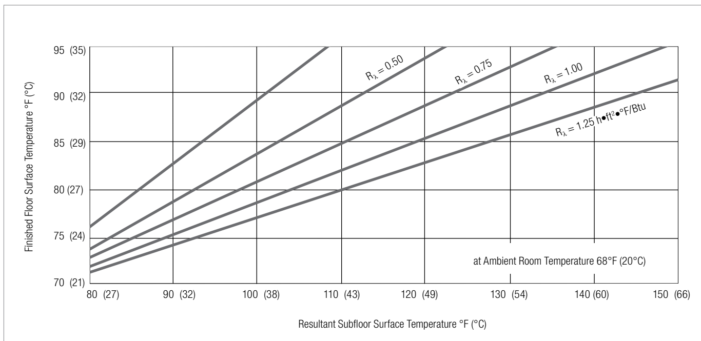
Fig. 6.1: Resultant subfloor surface temperature
