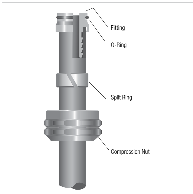
Fig. 4.5: R20 connection to manifold
