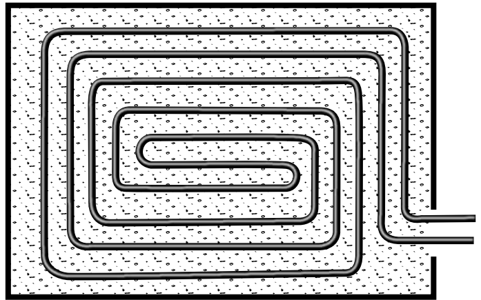
Fig. 6.6: Counter flow spiral pipe layout
