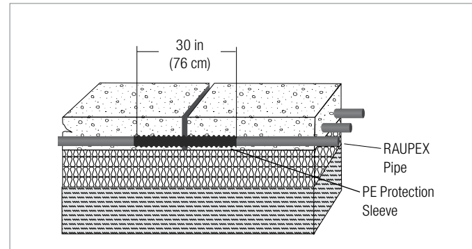
Fig. 5.6: Protective sleeving through movement joint
