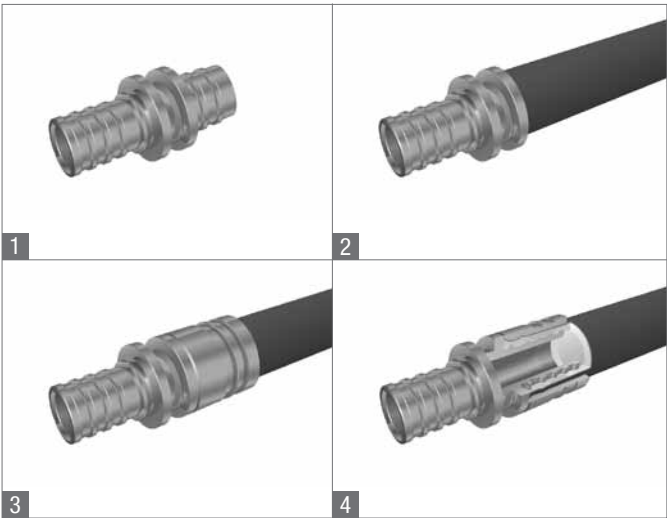
Fig. 4.4: (1) EVERLOC fitting, (2) fitting inserted in expanded pipe, (3) REHAU EVERLOC joint, (4) cutaway
