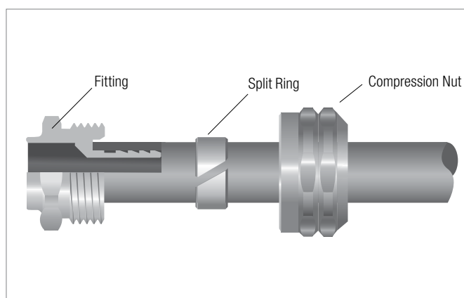
Fig. 4.6: Adapter connection to copper pipe
