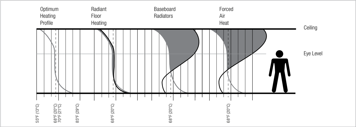
Fig. 3.1: Optimum heating distribution compared to representative temperature profiles for radiant, baseboard and forced-air heating.
