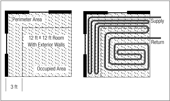
Fig 6.4: Overpour with perimeter and occupied areas using one circuit
