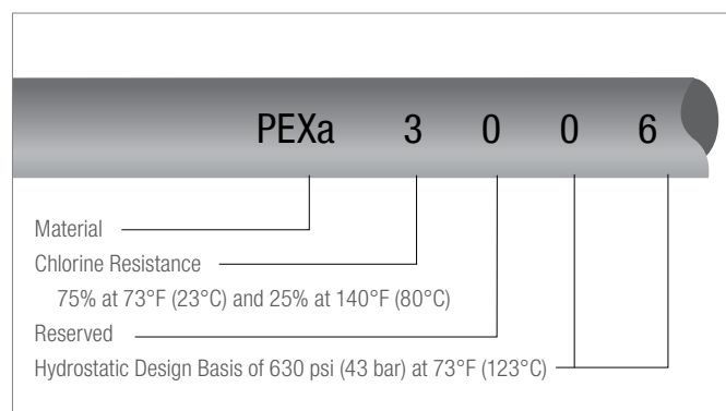
Fig. 4.2: Example RAUPEX O 2 Barrier Pipe Material Designation Code
