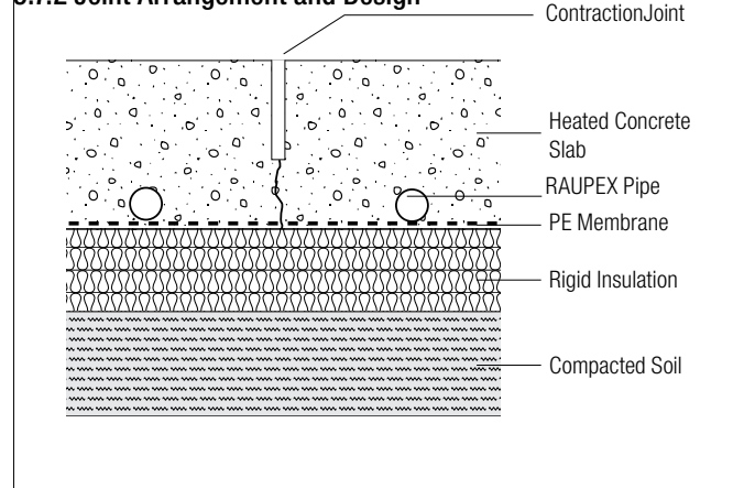
Fig. 5.3: Contraction joint
