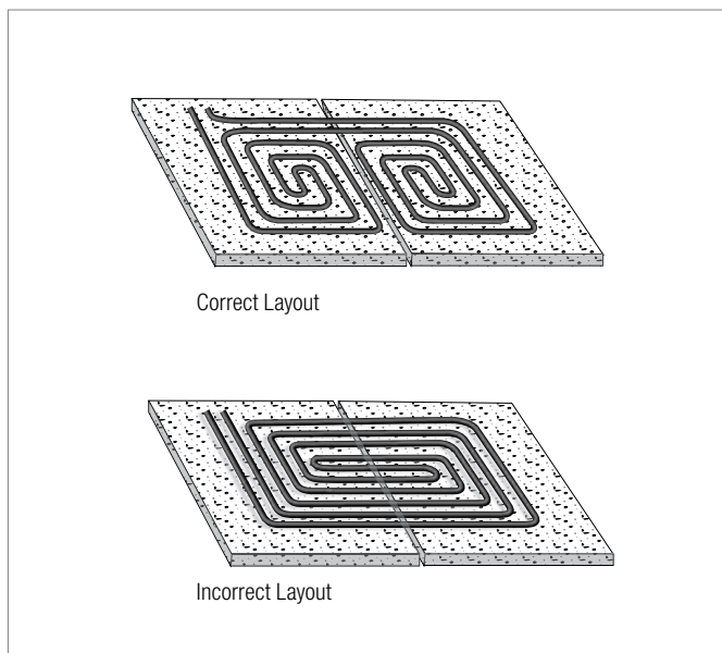
Fig. 5.5: Layout of radiant heating pipe with a thermal mass joint
